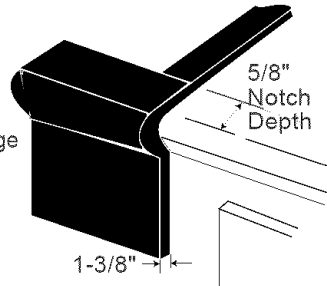
FIG. 6 Projecting from Cabinet Front
