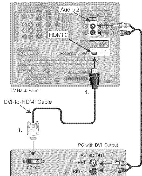
Figure 14. Connecting a Computer with DVI Monitor Output
