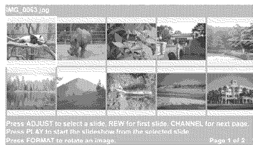
Figure 3. JPEG Thumbnails
