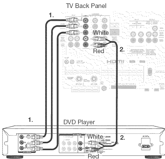
Figure 9. Connecting a DVD Player with Component Video
