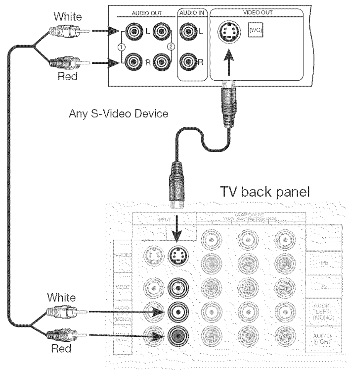
Figure 8. Connecting a Satellite Receiver with S-Video
