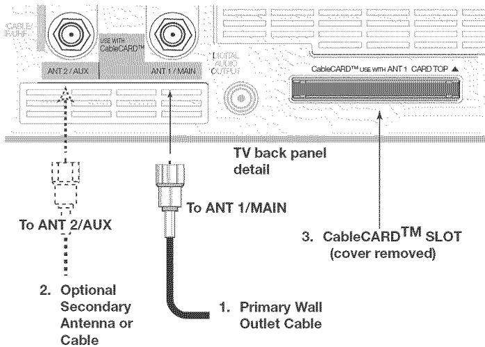
Figure 1. Wall Outlet Cable
