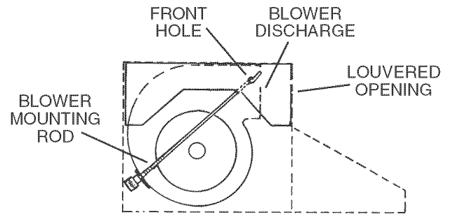
Non-ducted discharge - blower position
