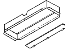
Non-Ducted Kit (For use with 3¼" x 10" Duct) (Includes 3¼" x 10" Damper & Vent Cover) Sears Part No. 59102
