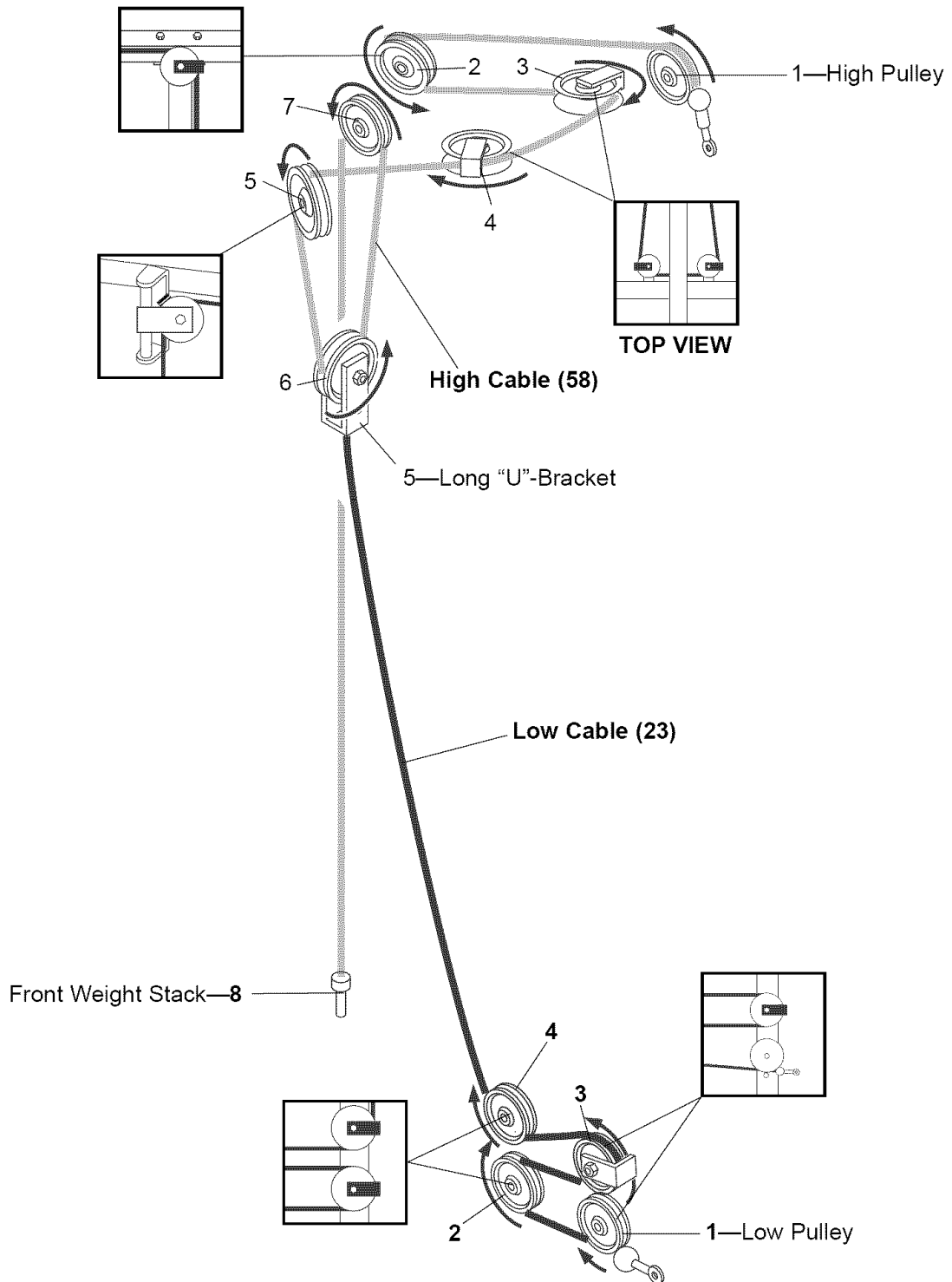
High Cable (58) and Low Cable (23)
