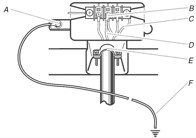
A. External ground conductor screw B. Center silver-colored terminal block screw C. Neutral grounding wire (green with yellow stripes) D. Neutral wire (white or center wire) E. 3/4" (1.9 cm) UL listed strain relief F. Grounding path determined by a qualified electrician
