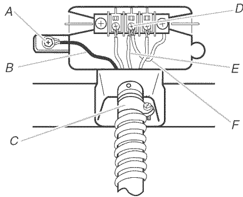
A. External ground conductor screw B. Ground wire (green or bare) of power supply cord C. 3/4" (1.9 cm) UL listed strain relief D. Center silver-colored terminal block screw E. Neutral wire (white or center wire) F. Neutral grounding wire (green with yellow stripes)
