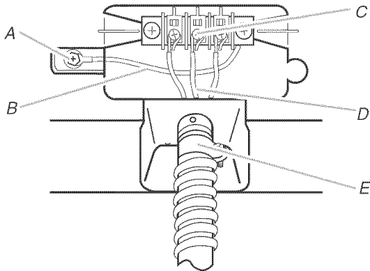
A. External ground conductor screw B. Neutral grounding wire (green with yellow stripes) C. Center silver-colored terminal block screw D. Neutral wire (white or center wire) E. 3/4" (1.9 cm) UL listed strain relief
