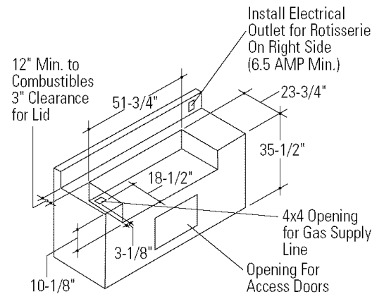
48" wide models: Installation in a combustible enclosure. ZX48JYSS insulated jacket is required.
