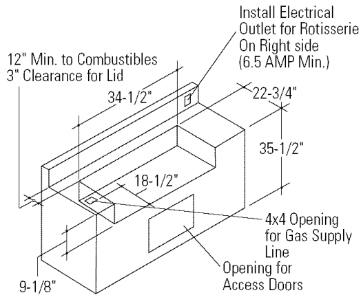
36" wide models: Installation in a non-combustible enclosure.
