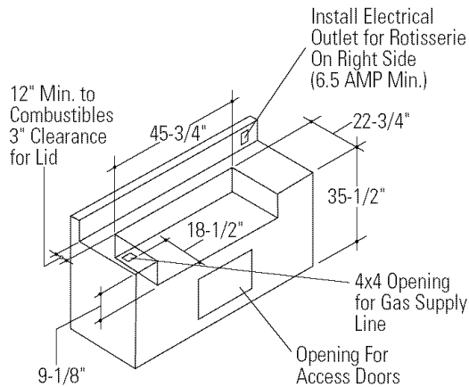
48" wide models: Installation in a non-combustible enclosure.
