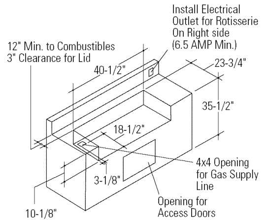
36" wide models: Installation in a combustible enclosure. ZX36JYSS insulated jacket is required.
