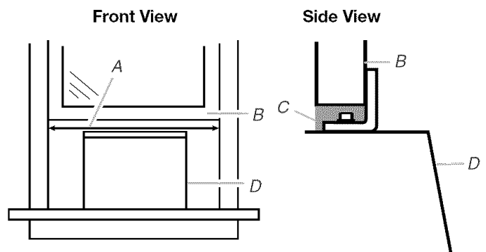
A. Width of frame B. Sash C. Foam window sash seal D. Cabinet
