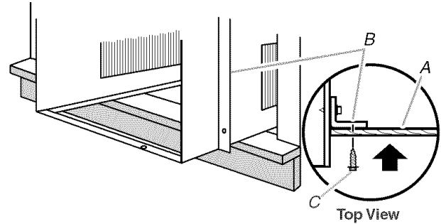
A. Right filler board B. Side-mounting angle C. \frac{1}{2} " hex-head screw
