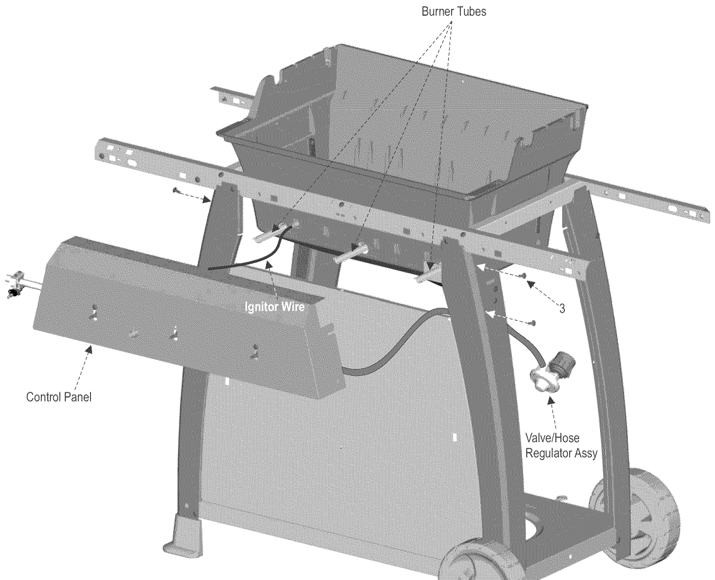
Correctly assembled burner tube and valve.
