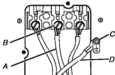
A. Neutral wire (white or center wire) B. Center terminal block screw C. External ground conductor screw D. Green or bare wire of power supply cable
