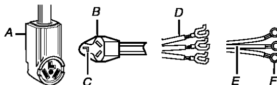
A. 3-wire receptacle (NEMA type 10-30R) B. 3-wire plug C. Neutral prong D. Spade terminals with upturned ends E. Neutral (white or center wire) F. Ring terminals
