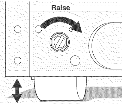
Adjusting Front Rollers.
