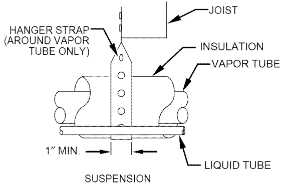
Fig. 2—Connecting Tubing Installation INSTALLATION
