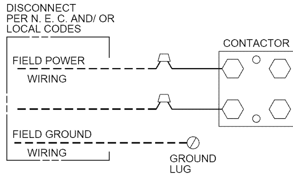
Fig. 12—Line Power Connections
