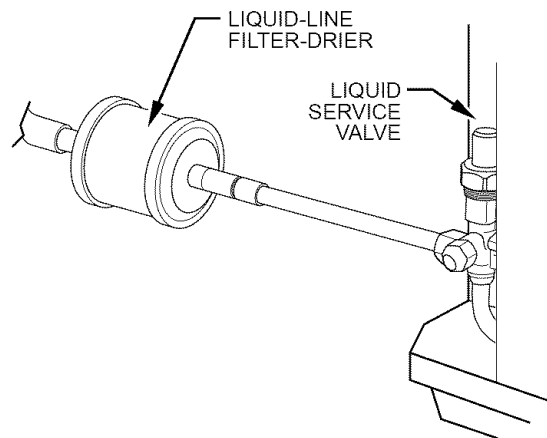
Fig. 9—Filter Drier with Sweat Adapter Tube and Liquid Tube
