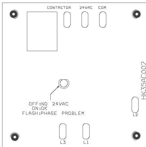
Fig. 10—Phase Monitor Control
