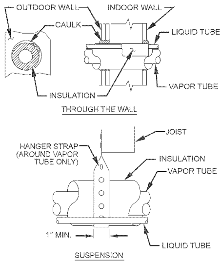
Fig. 2—Connecting Tubing Installation INSTALLATION
