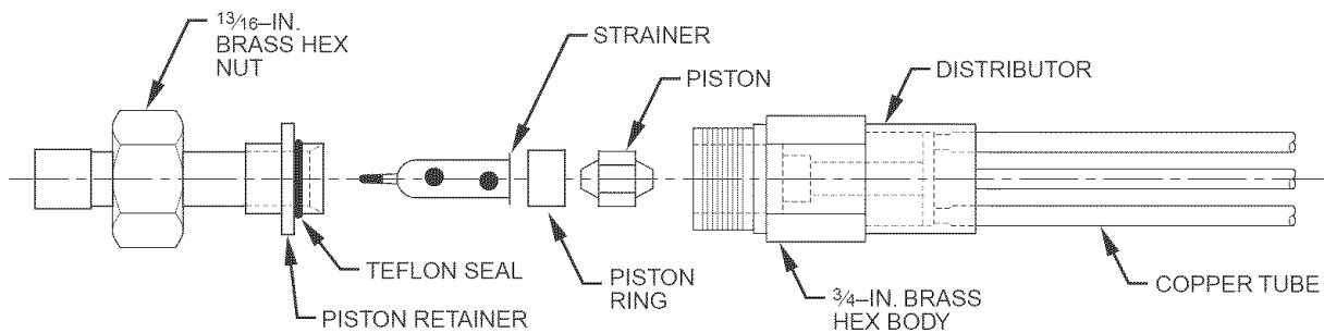
Fig. 4—AccuRater® Components (38EZG Use)
