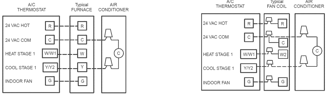
Fig. 11—Generic Wiring Diagram (See Thermostat Installation Instructions for wiring specific unit combinations)
