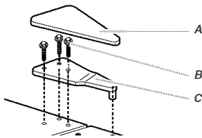
A. Top Hinge Cover B. \frac{1}{16} " Hex-Head Hinge Screws C. Top Hinge
