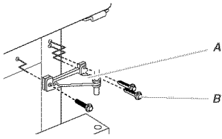
A. Center Hinge B. \frac{1}{16} " Hex-Head Hinge Screws
