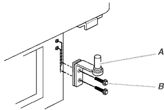
A. Bottom Hinge B. \frac{1}{16} " Hex-Head Hinge Screws
