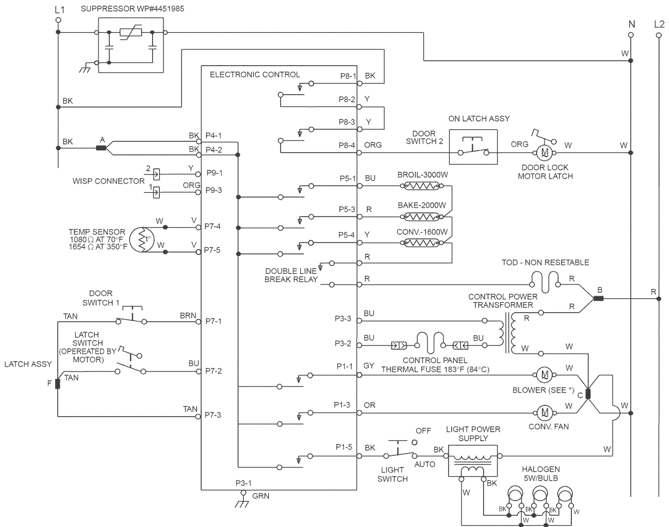
Oven schematic
