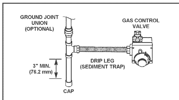
FIGURE 19. GAS PIPING WITH FLEXIBLE CONNECTOR.
