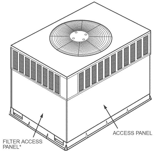
Fig. 2—Accessory Filter Rack Access Panel
