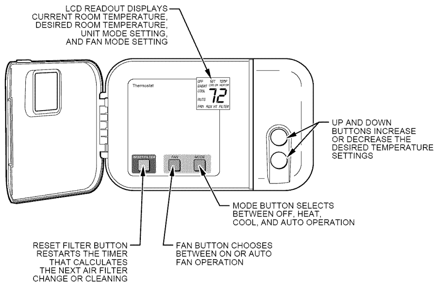
Fig. 2—Carrier Non-Programmable Thermostat
