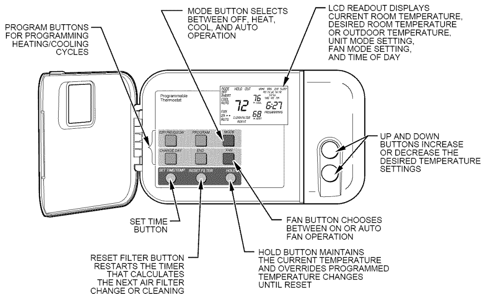
Fig. 3—Carrier Programmable Thermostat
