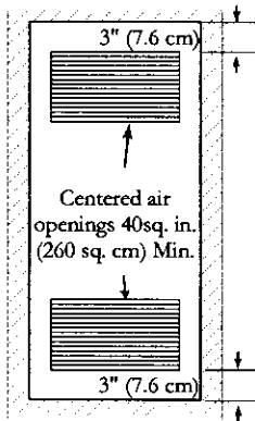
FRONT VIEW (Closet Door)
