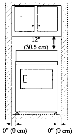
FRONT VIEW (w/o Closet Door)
