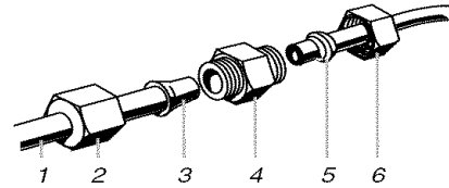
1. Line to refrigerator 4. Coupling (provided) 2. Nut (provided) 5. Ferrule (purchased) 3. Bulb 6. Nut (purchased)
