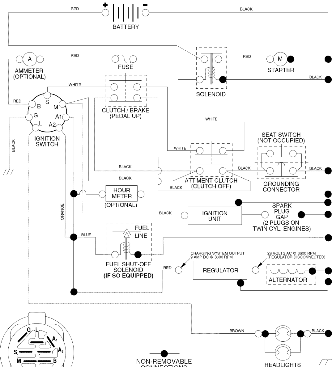
IGNITION SWITCH
