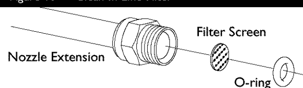
Figure 10 — Clean In-Line Filter
