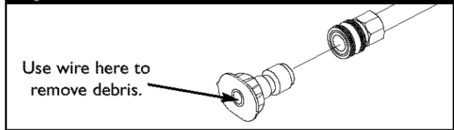
Figure 11 — Nozzle Maintenance
