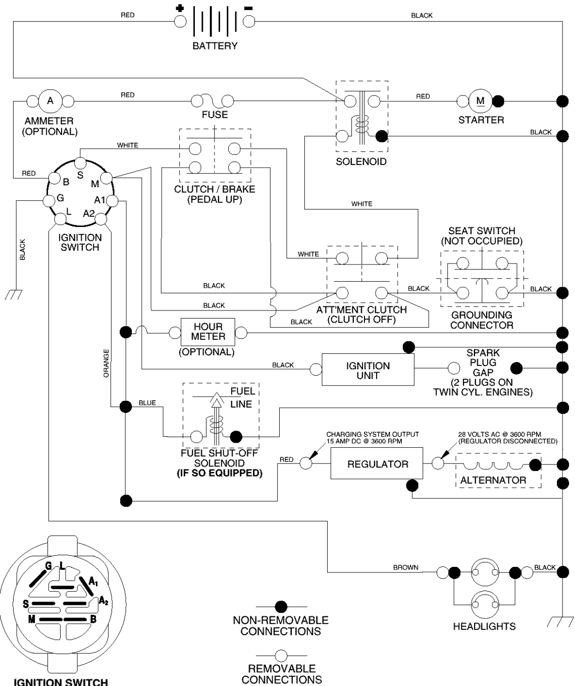
IGNITION SWITCH
