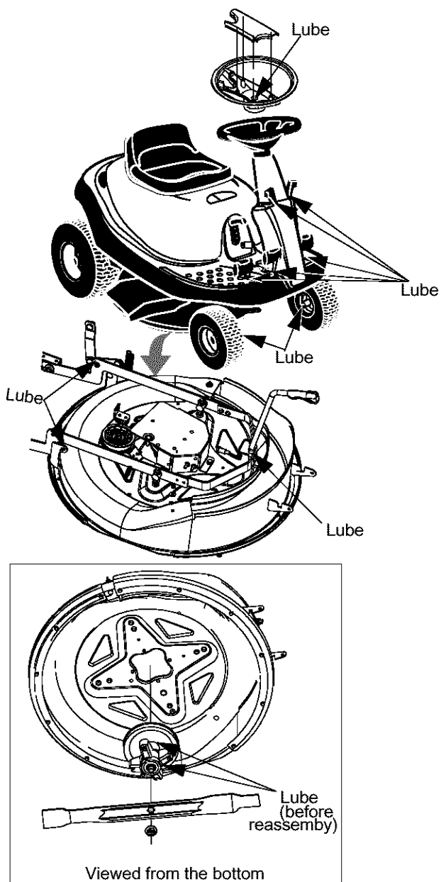
Figure 19: Lubrication Chart
