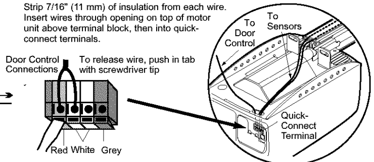
Figure 3 Wiring to Terminal Block
