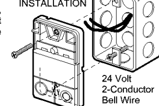
Figure 3 Wiring to Terminal Block
