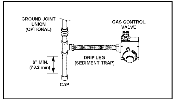
FIGURE 19. GAS PIPING WITH FLEXIBLE CONNECTOR.
