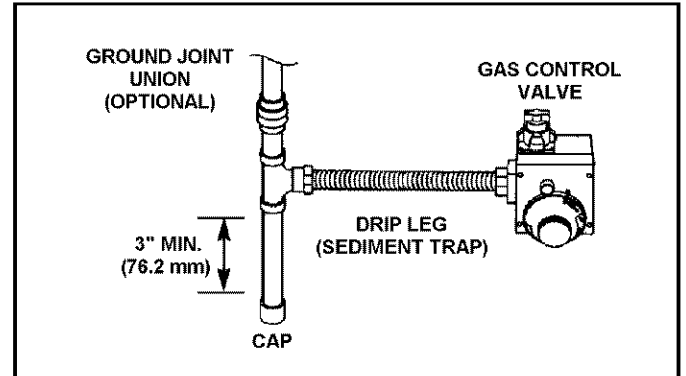
FIGURE 19. GAS PIPING WITH FLEXIBLE CONNECTOR.
