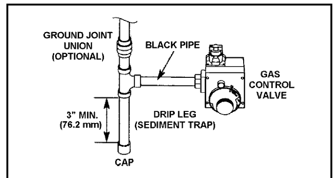
FIGURE 20. GAS PIPING WITH ALL BLACK IRON PIPE TO GAS CONTROL.
