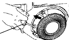
Rewind Starter
