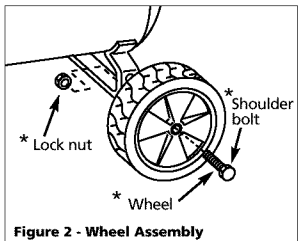
Figure 2 - Wheel Assembly
