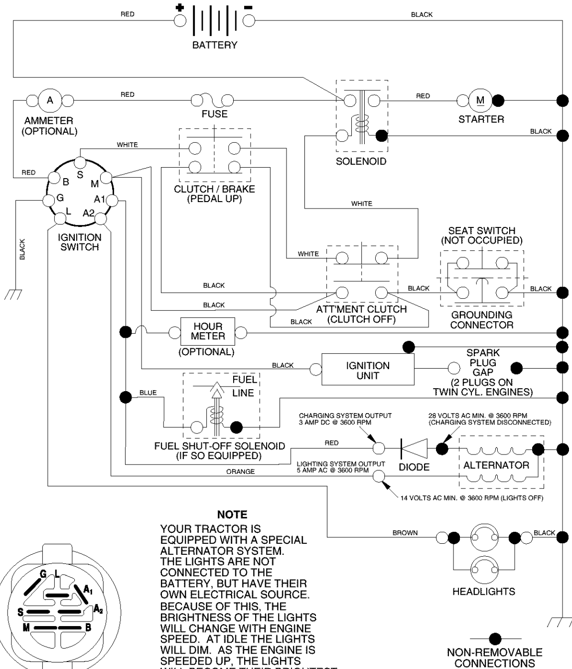
IGNITION SWITCH
