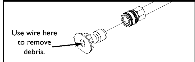
Figure 18 — Nozzle Maintenance
