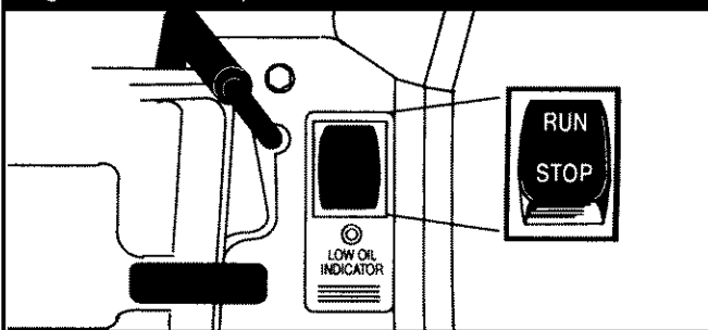
Figure 7 — Run/Stop Switch
