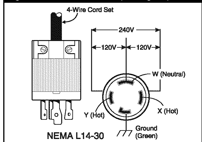
Figure 11 — 120/240 Volt AC, 30 Amp, Locking Receptacle
