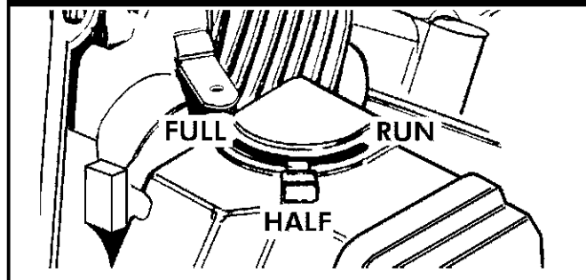
Figure 8 — Choke Lever
