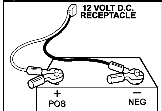
Figure 9 — Battery Connections
