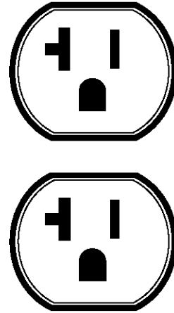
Figure 8 — 120 Volt, 20 Amp Duplex Receptacle
