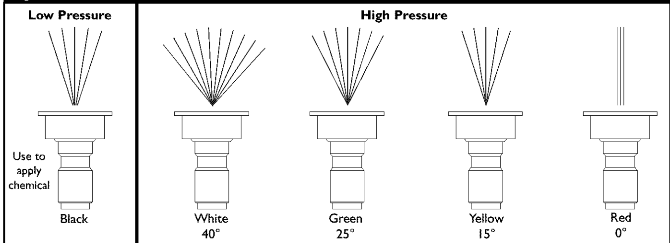
Figure 17 — Nozzles
