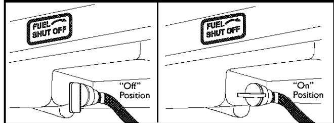
Figure 4 — Fuel Valve
