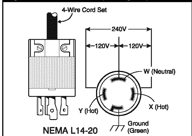
Figure 8 — 120/240 Volt, 20 Amp Locking Receptacle
