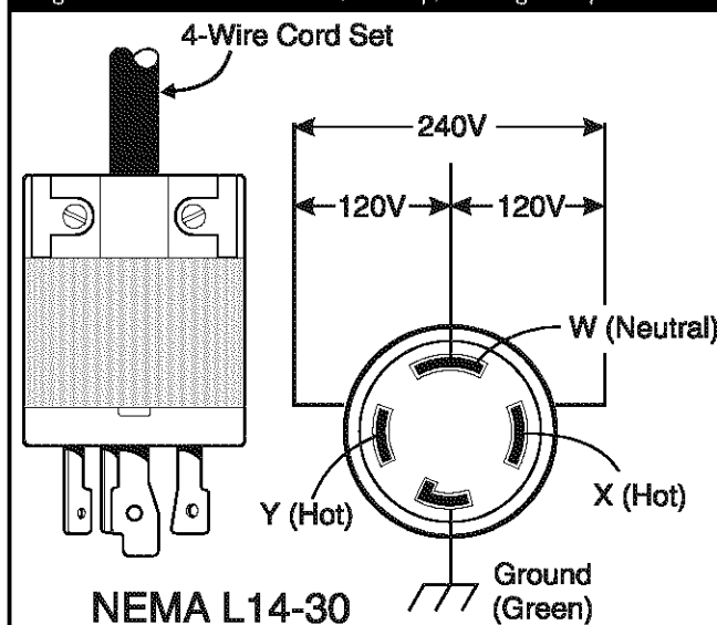
Figure 8 — 120/240 Volt AC, 30 Amp, Locking Receptacle
