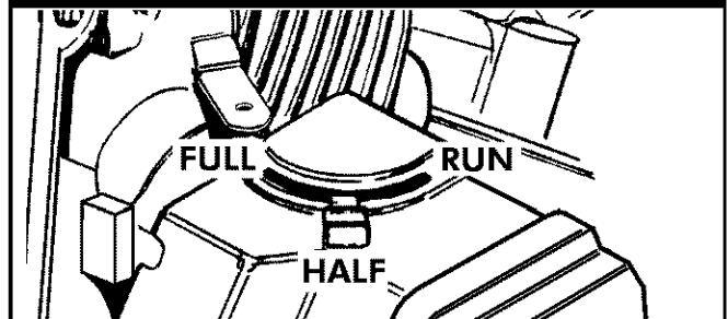
Figure 5 — Choke Lever
