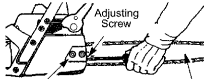
Chain Brake Nuts Adjusting Screw Guide Bar
