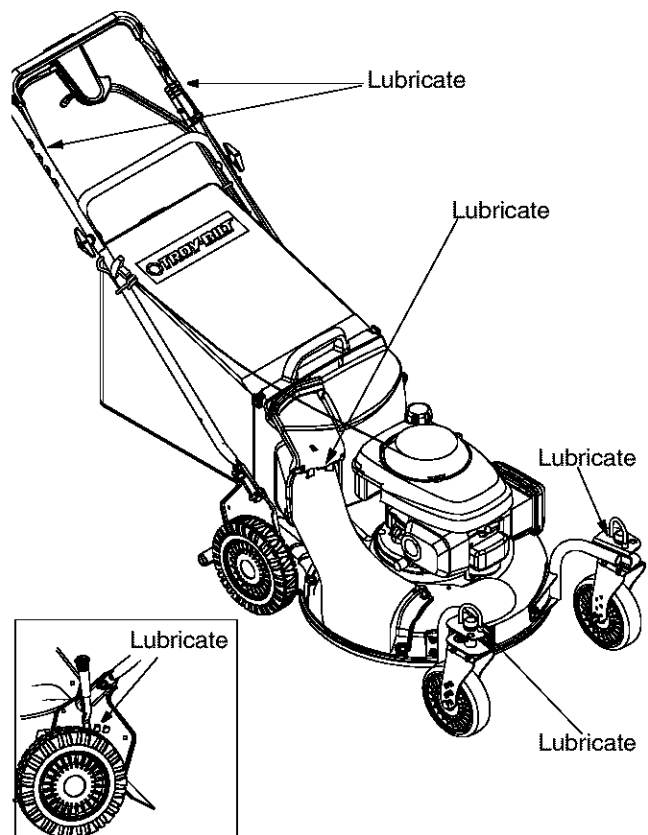
Figure 17: Lubrication Chart
