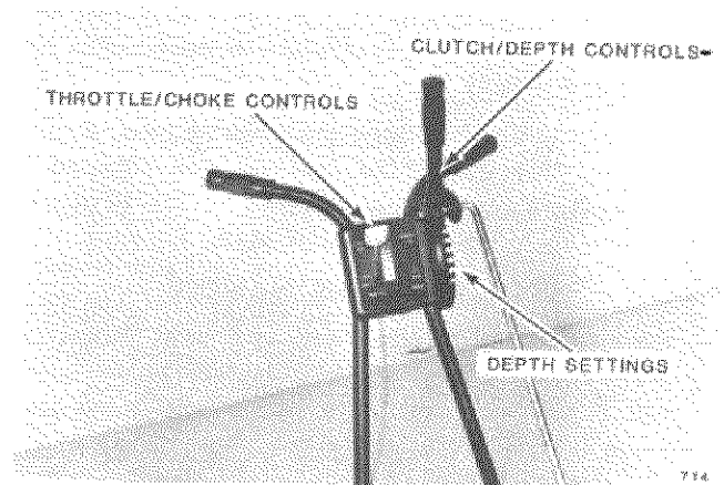
Throttle/Choke and Clutch/Depth Controls.
