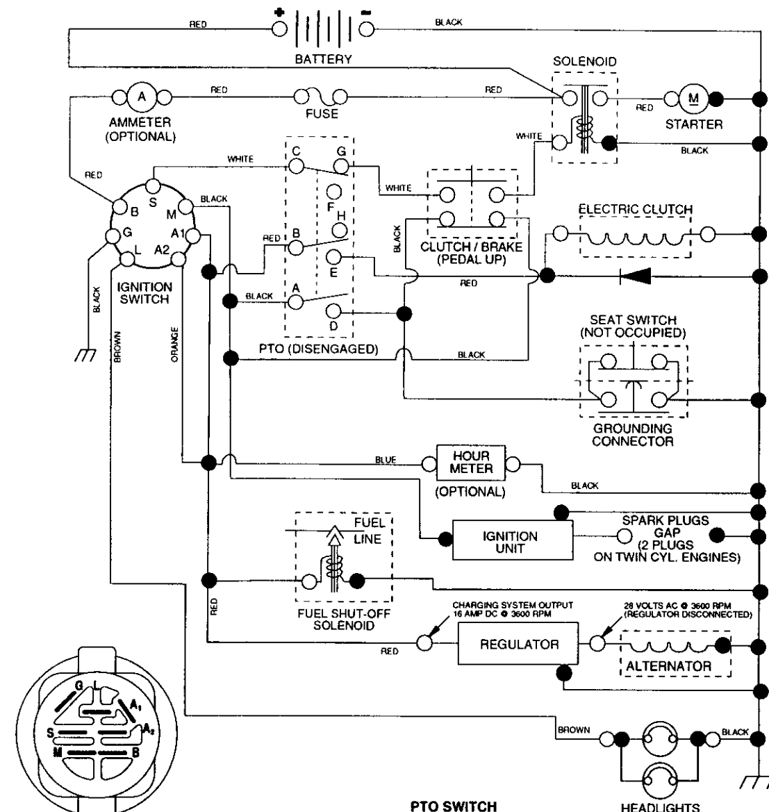
IGNITION SWITCH
