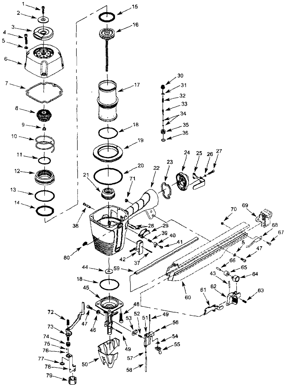
Figure 12 - Replacement Parts Illustration For Framing Nailer
