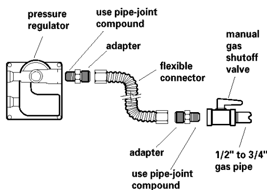
Typical flexible connection
