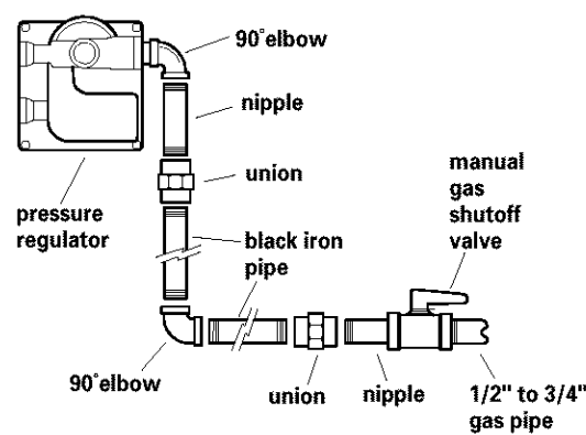
Typical rigid pipe connection
