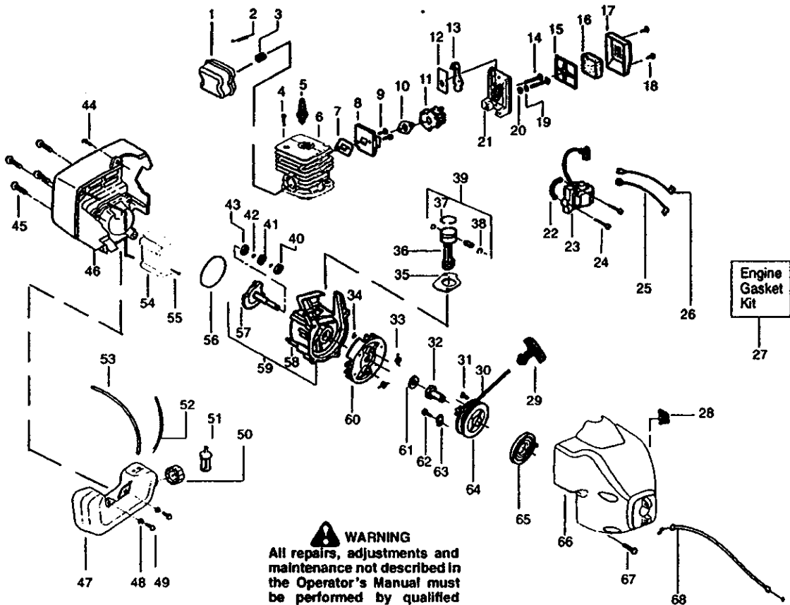
SEARS TRIMMER MODEL 358.794251
