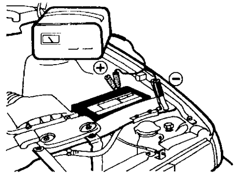
NEGATIVE GROUNDED SYSTEM Figure A
