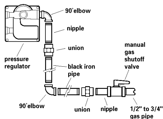
Typical rigid pipe connection
