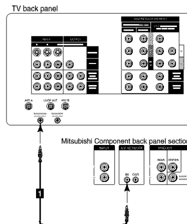
Figure 1. Connecting the Active A/V Network.
