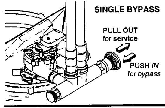
3 - VALVE BYPASS
