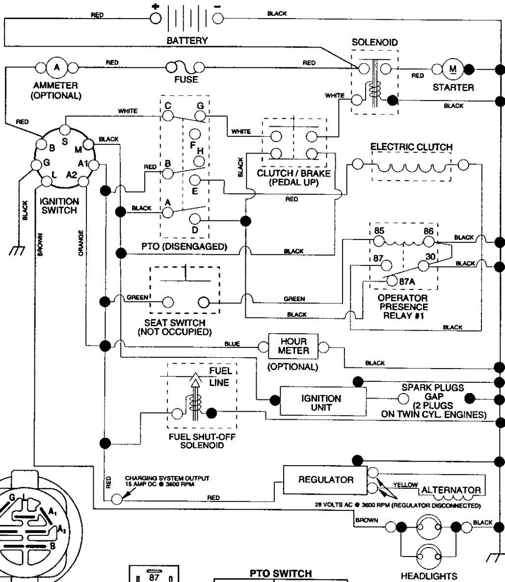
IGNITION SWITCH
